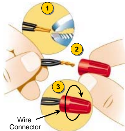
Figure 5.2 Wires splicing
